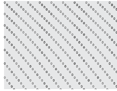
TV55 (exit density 550) for fine counts, for medium counts with the highest quality requirements and for medium and fine counts on high speed cards
