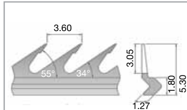
VH20/360/55 SiroLock®
