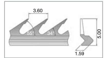
VH16/360/55 SiroLock®
