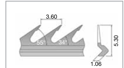
VL24/360/55 SiroLock®
