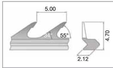
VH12/500/55 SiroLock®
