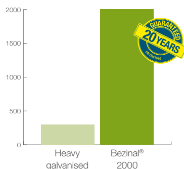
(Hours salt spray before 5% DBR)
